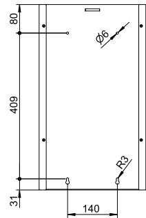
Bohrbild | drilling pattern
