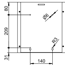
Bohrbild | drilling pattern
