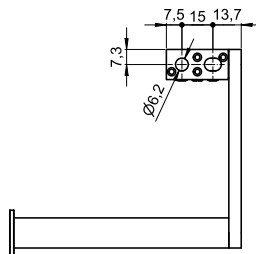
Bohrbild | drill pattern
