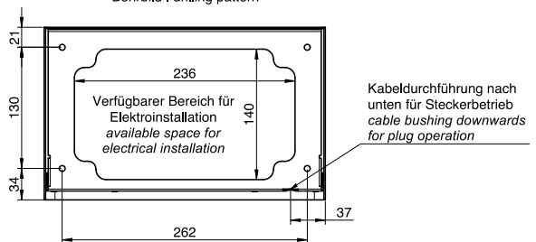
Bohrbild I drilling pattern
